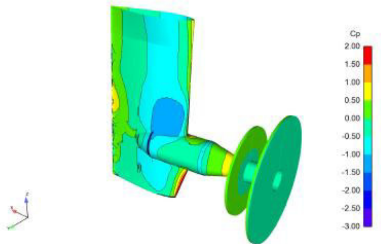
Figure 3.1.3.2.- First option strut calculated with CFD
